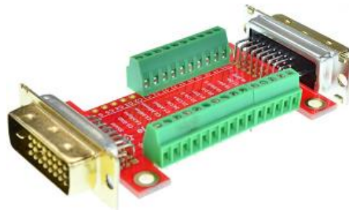
Figure 4: DVI-DM-DM-V1A with terminal block
